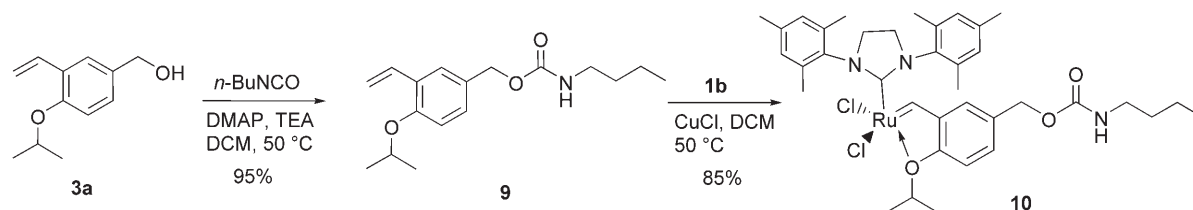
Scheme 2. Synthesis of homogeneous carbamate catalyst 10 .
