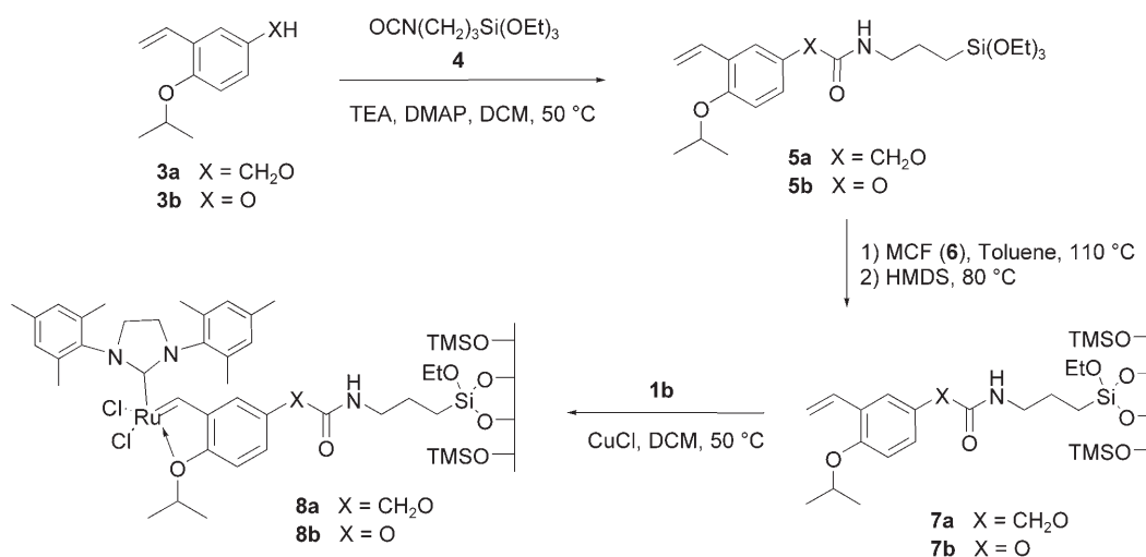
Scheme 1. Synthesis of the heterogenized ruthenium catalysts 8 .
