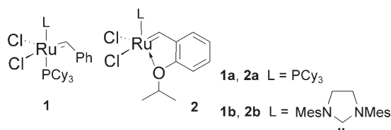
Figure 1. Structures of the ruthenium catalysts.
